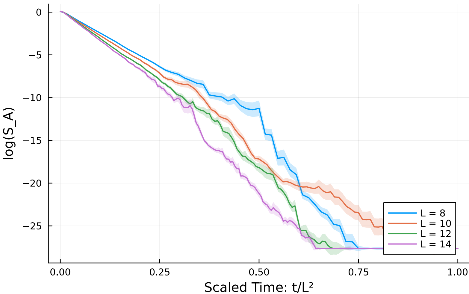
Scaled Log Entropy Evolution ( p = 0.600000 )
